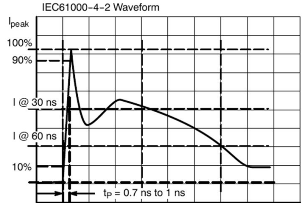
Figure 1: IEC61000-4-2 Waveform
